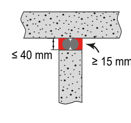
EI90-T-X-F-W5 to 40
