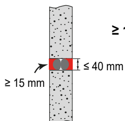
EI90-V-X-F-W5 to 40
